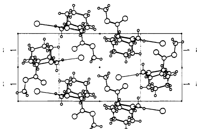
Figure 2. The unit cell, viewed along the c axis. The long axis is b . A line connects each iodide ion with its nearest sulfur neighbor.
