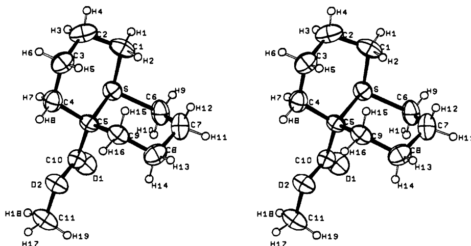
Figure 1. Stereodrawing (ORTEP) of the bicyclic sulfonium cation 9 . Hydrogen atoms are drawn with fictitious spherical thermal parameters of 0.5 \text{ \AA}^2 .
