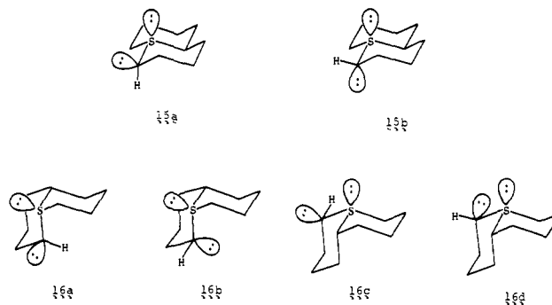
Figure 3. Possible conformations of ylides 15 and 16 .
